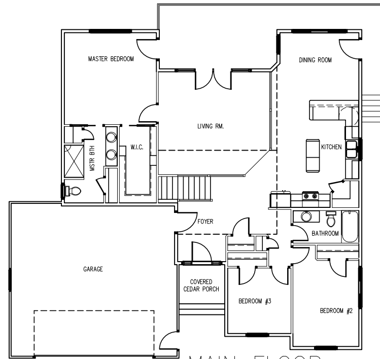
MAIN FLOOR 1645 SQ.FT.
