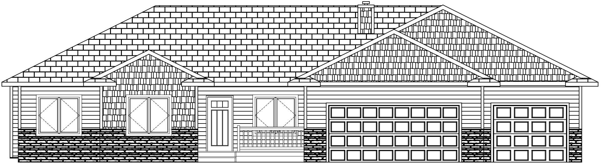
CHAMBERLAIN FRONT ELEVATION
